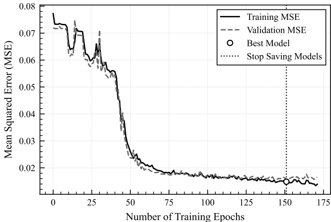
Learning Curve of MHSA-LSTM Model for SolarPlant-3 (Gyeongju)
